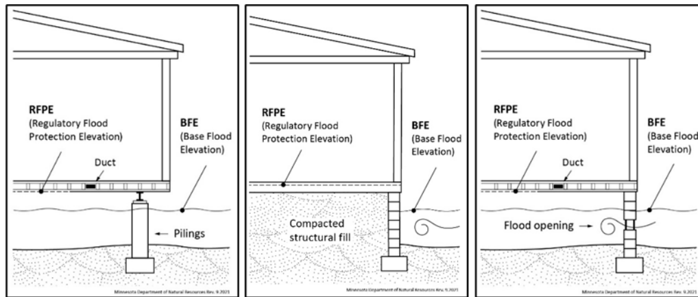
Figure 6: Internally flooded enclosed area.
